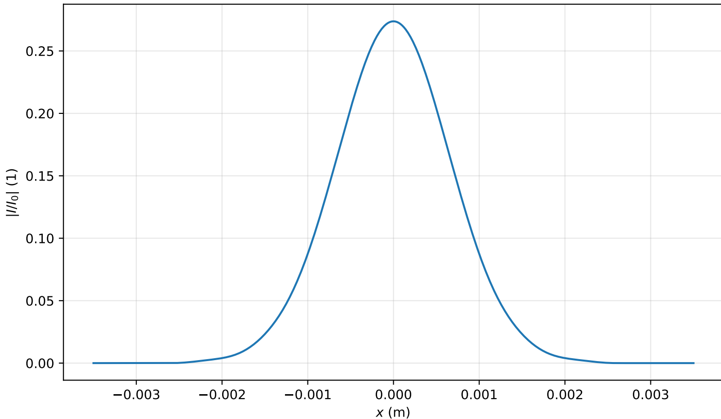
Intensity profile I(x, y = 0, z = 3.742m)/I_0 , P_{in}=0.2P_{cr} , artificial time
